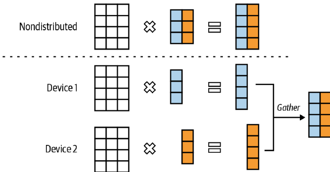
Figure 9-18. Tensor parallelism for matrix multiplication.
