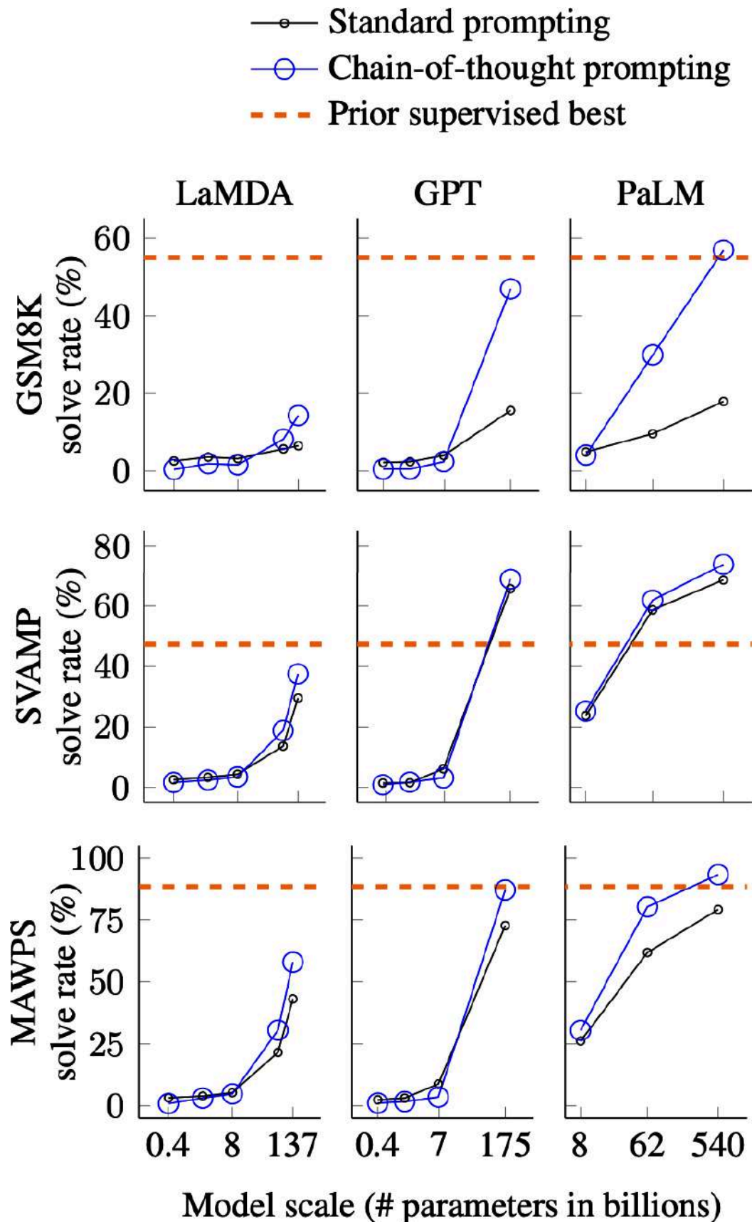
Figure 5-6. CoT improved the performance of LaMDA, GPT-3, and PaLM on MAWPS (Math Word Problem Solving), SVAMP (sequence variation analysis, maps, and phylogeny), and GSM-8K benchmarks. Screenshot from Wei et al., 2022. This image is licensed under CC BY 4.0.
