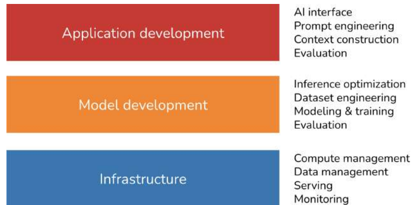
Figure 1-14. Three layers of the AI engineering stack.
