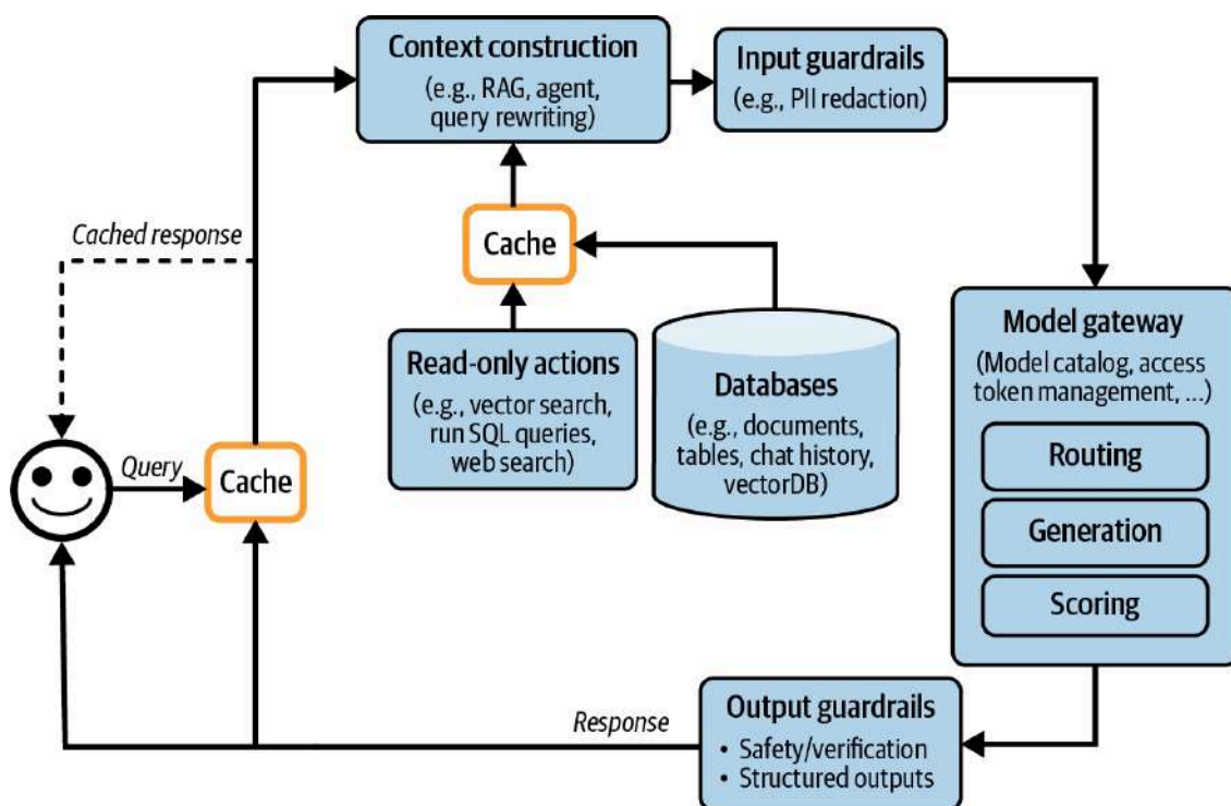
Figure 10-8. An AI application architecture with the added caches.
