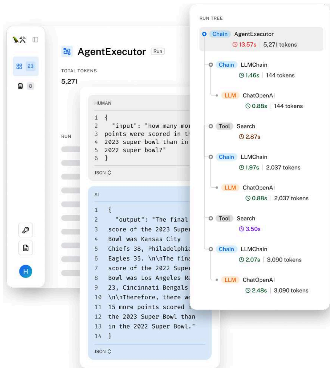
Figure 10-11. A request trace visualized by LangSmith.
