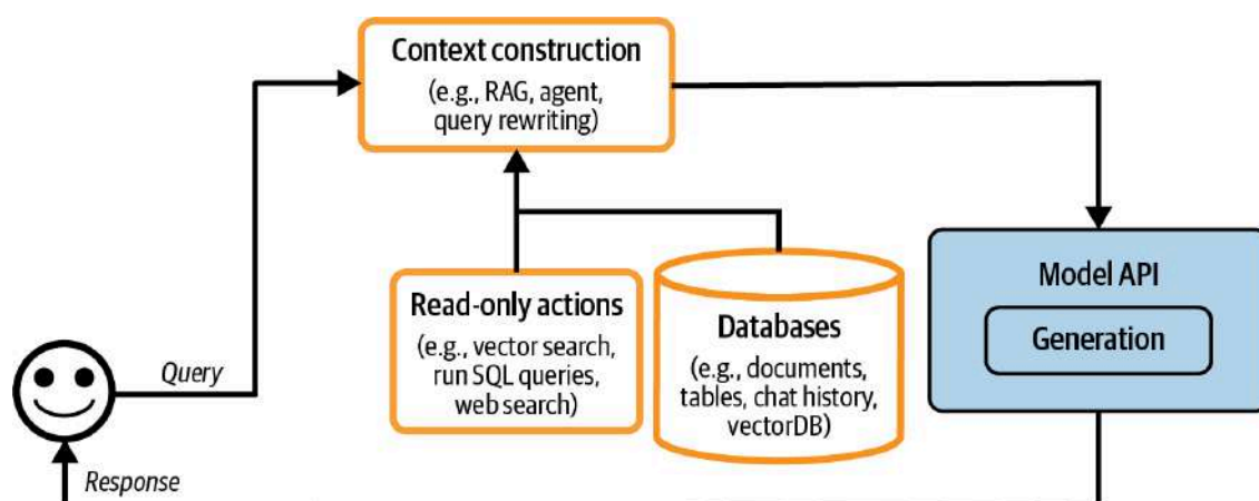
Figure 10-2. A platform architecture with context construction.
