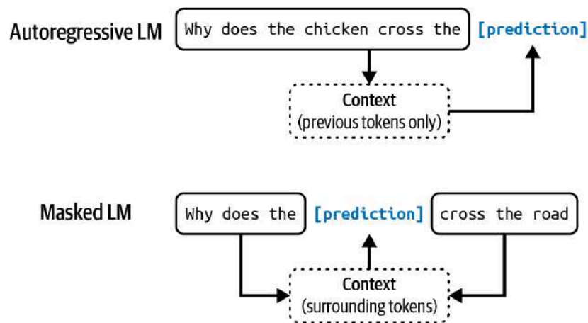
Figure 1-2. Autoregressive language model and masked language model.
