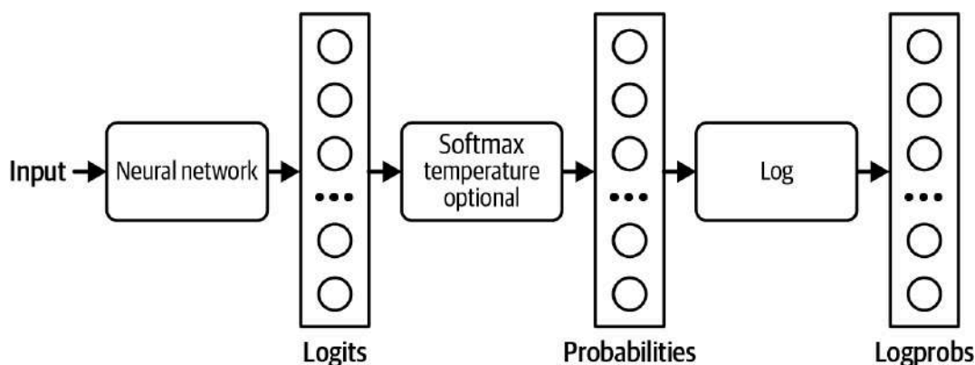
Figure 2-17. How logits, probabilities, and logprobs are computed.
